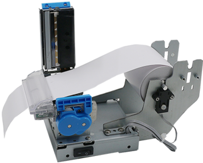
EP602-TM 60mm ticket/receipt/label printer
